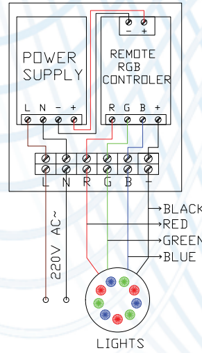
4 WIRES SYSTEM
